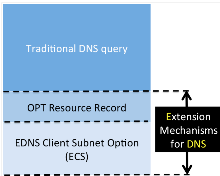
Figure 1. How the traditional DNS query can be extended
