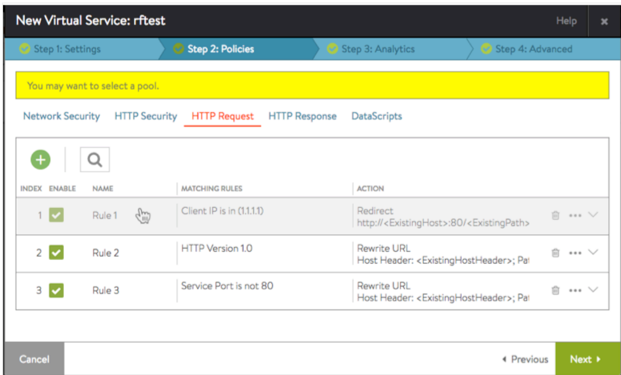
Figure 2. Virtual service advanced setup wizard with three rules in numerical sequence
