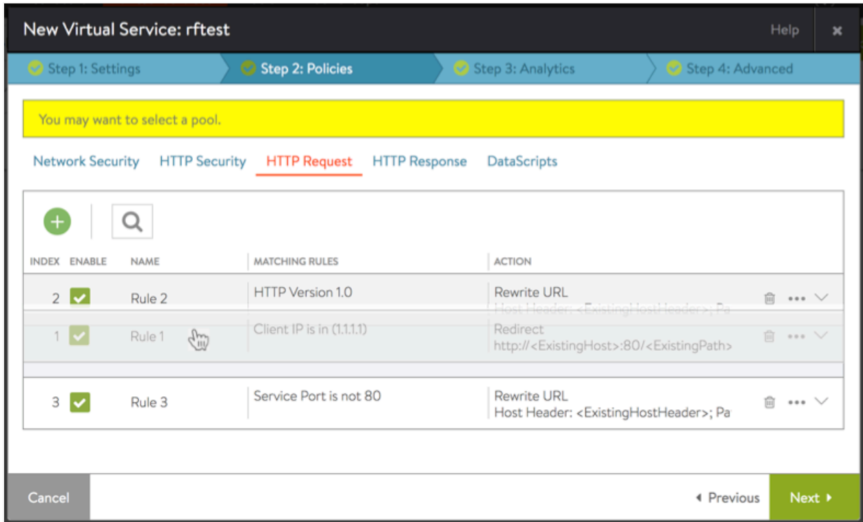
Figure 3. Rule 1 is being dragged downward
